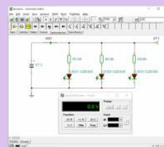
Fig. 2: parallel circuit 2
