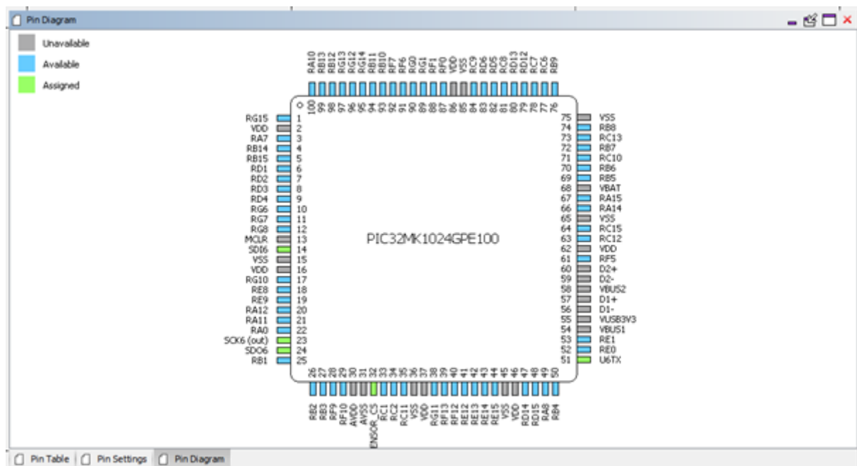
Abb. 29: Harmony Pin Diagram
